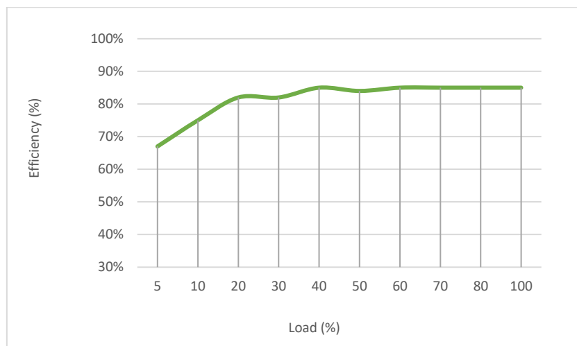
SDU06D2405, with nominal input voltage
