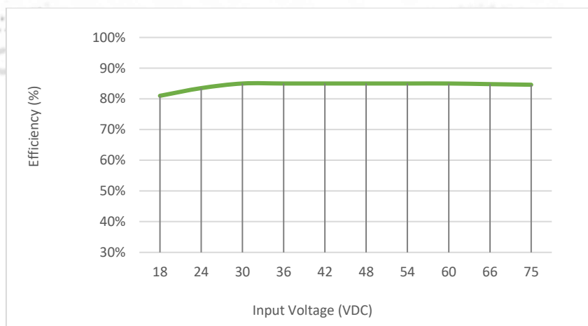
SDU06D4815D, with full Load
