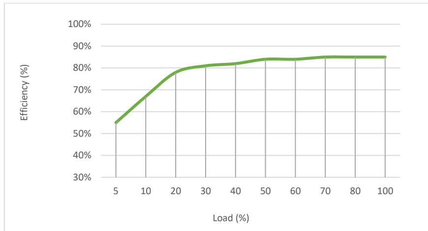
SDU06GD4815D, with nominal input voltage
